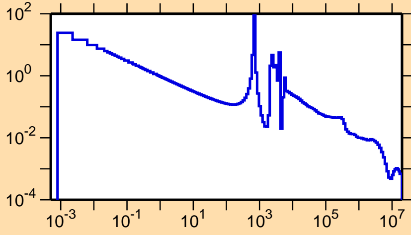
\sigma vs. E for ^{102}\text{Mo}(n,\gamma)
