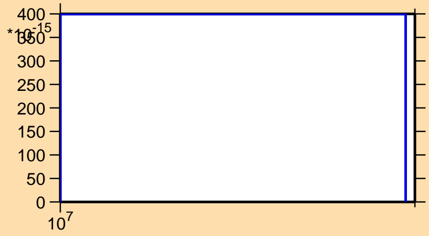
\sigma vs. E for ^{102}\text{Mo}(n,nd)
