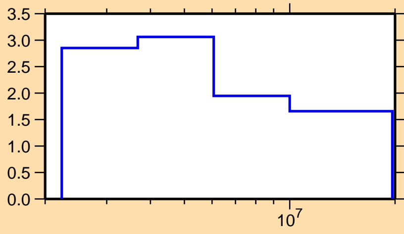
\Delta\sigma/\sigma vs. E for ^{102}\text{Mo}(n,n\text{onel.})
