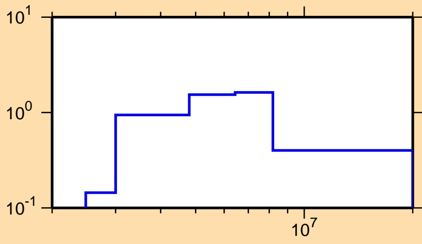
\sigma vs. E for ^{102}\text{Mo}(n,n\text{cont.})
