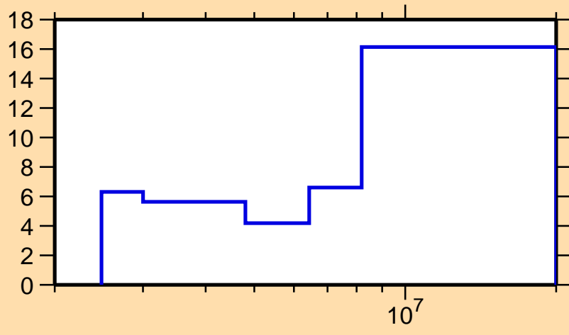
\Delta\sigma/\sigma vs. E for ^{102}\text{Mo}(n,n\text{cont.})
