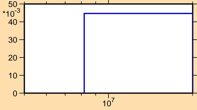
\sigma vs. E for ^{102}\text{Mo}(n,3n)
