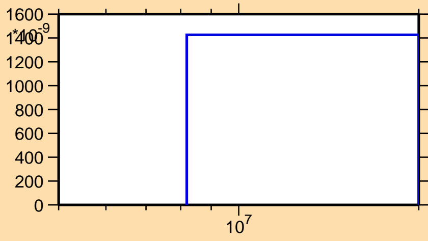
\sigma vs. E for ^{102}\text{Mo}(n,t)
