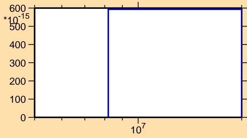
\sigma vs. E for ^{102}\text{Mo}(n,\text{nd})
