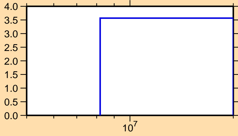
\Delta\sigma/\sigma vs. E for ^{102}\text{Mo}(n,2n)
