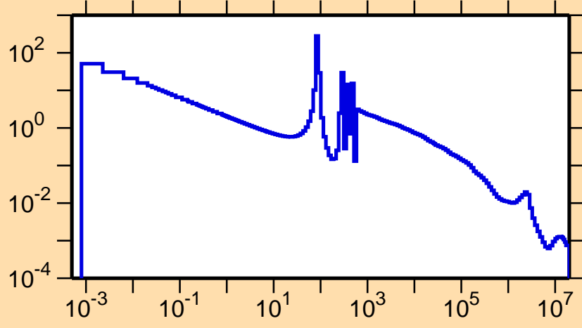
\sigma vs. E for ^{103}\text{Mo}(n,\gamma)
