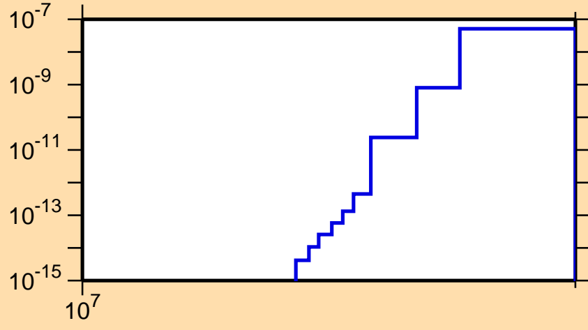
\sigma vs. E for ^{103}\text{Mo}(n,2n\alpha)
