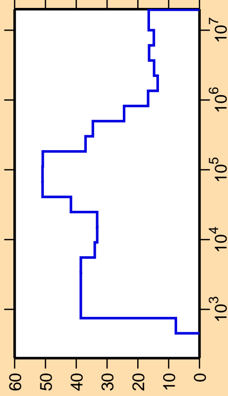
\Delta\sigma/\sigma vs. E for ^{103}\text{Mo}(n,\text{nonel.})
