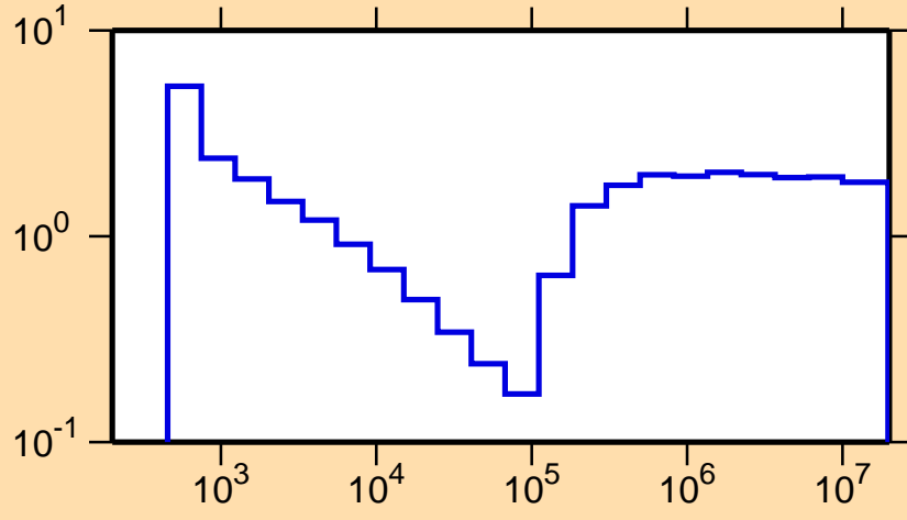
\sigma vs. E for ^{103}\text{Mo}(n,\text{nonel.})
