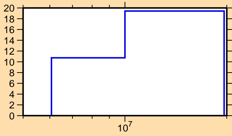
\Delta\sigma/\sigma vs. E for ^{103}\text{Mo}(n,el.)
