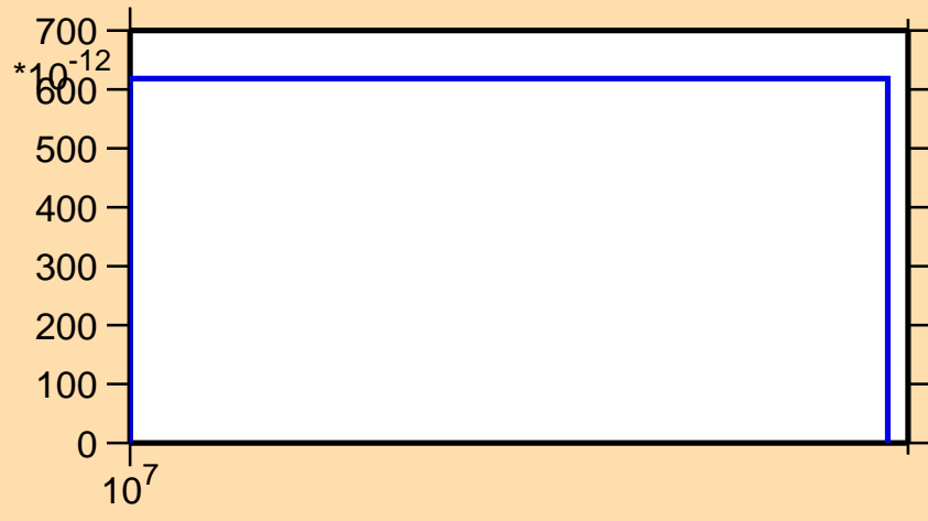
\sigma vs. E for ^{103}\text{Mo}(n,\text{nd})
