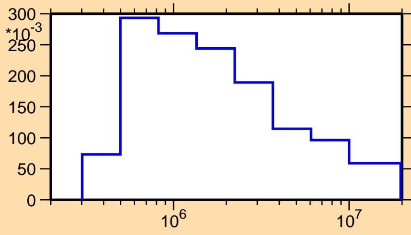
\sigma vs. E for ^{103}\text{Mo}(n,n_4)
