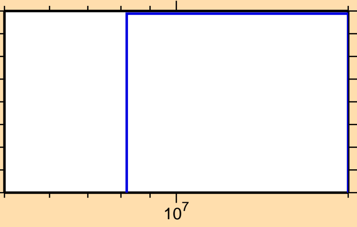
\sigma vs. E for ^{103}\text{Mo}(n,\text{nd})
