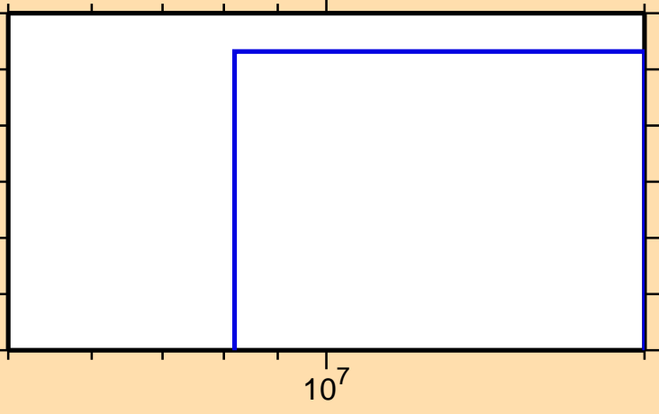
\sigma vs. E for ^{103}\text{Mo}(n,n\alpha)
