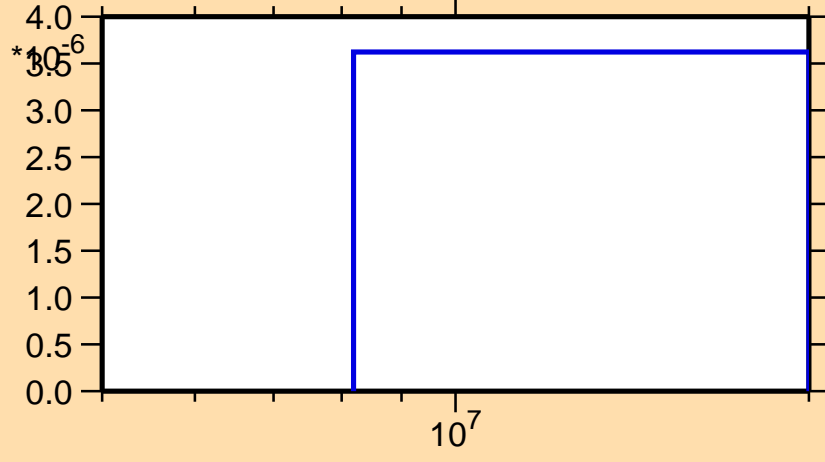
\sigma vs. E for ^{103}\text{Mo}(n,t)
