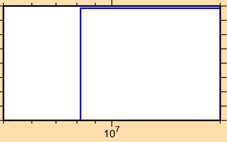
\sigma vs. E for ^{103}\text{Mo}(n,d)
