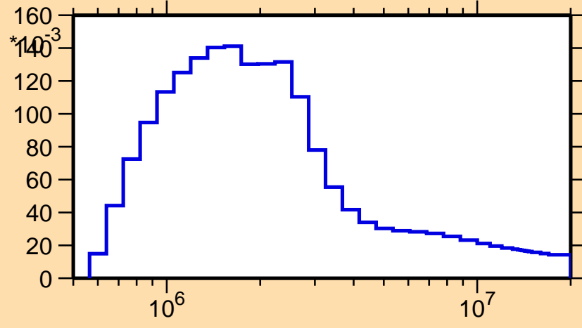
\sigma vs. E for ^{104}\text{Mo}(n,n_2)
