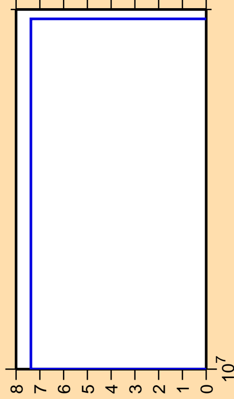
\Delta\sigma/\sigma vs. E for ^{104}\text{Mo}(n,nt)
