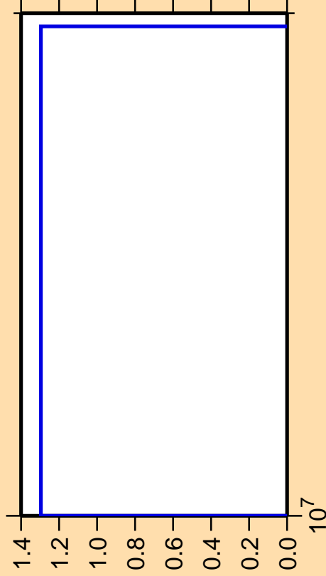
\Delta\sigma/\sigma vs. E for ^{104}\text{Mo}(n,nd)
