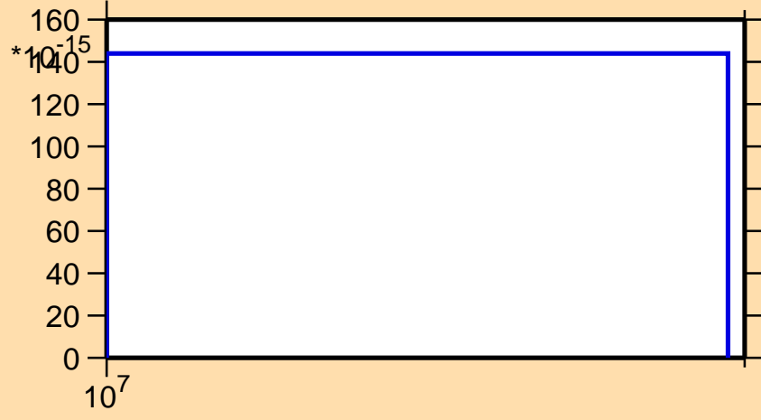
\sigma vs. E for ^{104}\text{Mo}(n,nd)
