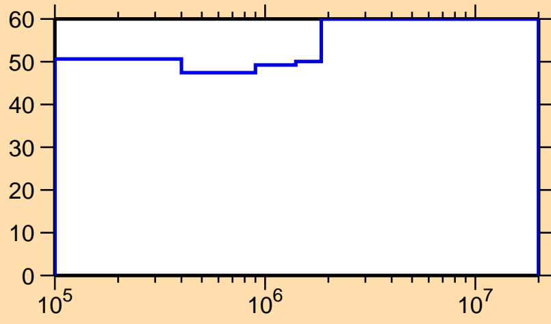
\Delta\sigma/\sigma vs. E for ^{104}\text{Mo}(n,n_1)
