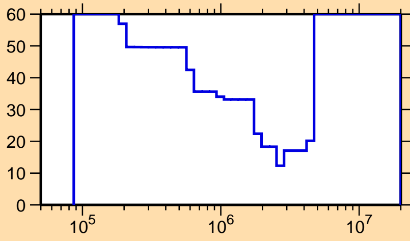
\Delta\sigma/\sigma vs. E for ^{105}\text{Mo}(n,\text{inel.})
