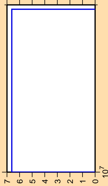
\Delta\sigma/\sigma vs. E for ^{105}\text{Mo}(n,2n\alpha)
