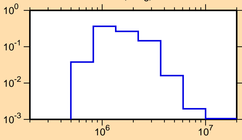
\sigma vs. E for ^{106}\text{Mo}(n,n_3)
