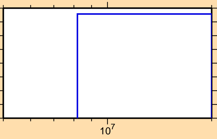
\sigma vs. E for ^{106}\text{Mo}(n,d)
