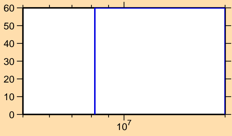
\Delta\sigma/\sigma vs. E for ^{106}\text{Mo}(n,ncont.)
