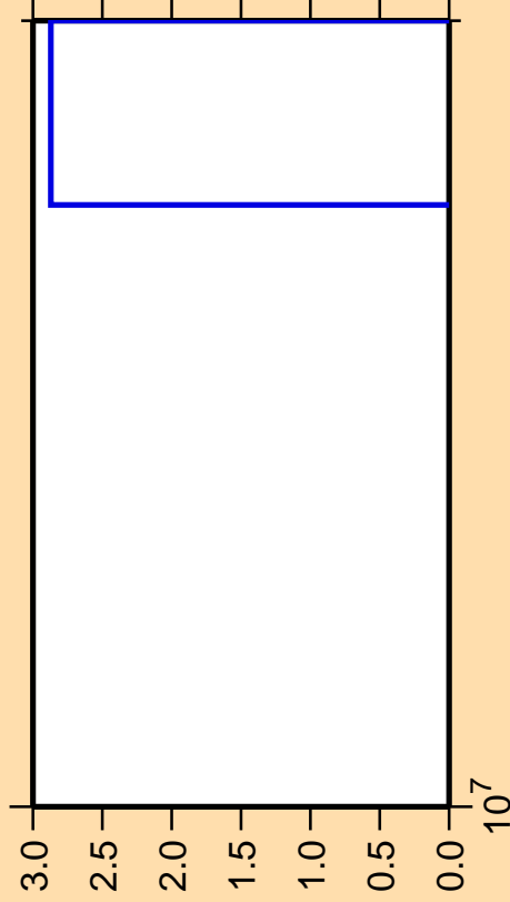
\Delta\sigma/\sigma vs. E for ^{108}\text{Mo}(n,nd)
