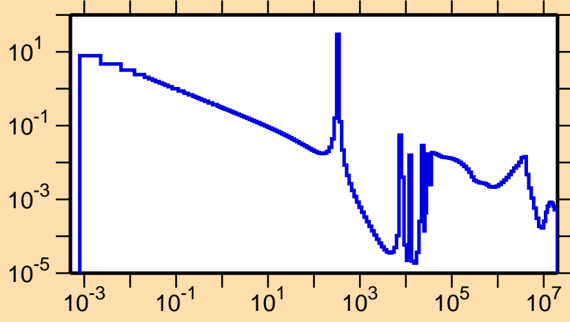
\sigma vs. E for ^{108}\text{Mo}(n,\gamma)
