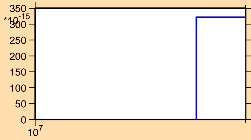
\sigma vs. E for ^{108}\text{Mo}(n,nd)
