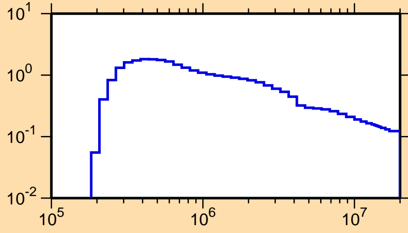
\sigma vs. E for ^{108}\text{Mo}(n,n_1)
