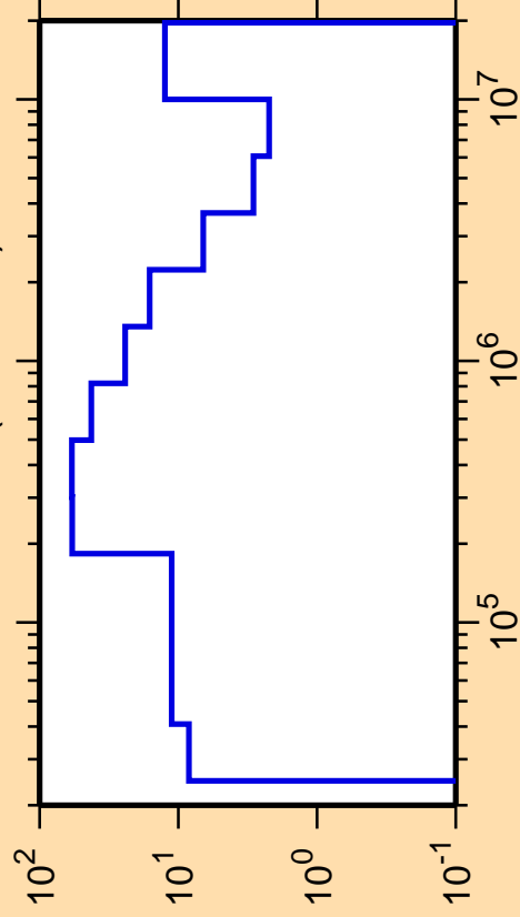
\Delta\sigma/\sigma vs. E for ^{108}\text{Mo}(n,\text{nonel.})
