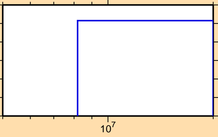
\sigma vs. E for ^{108}\text{Mo}(n,np)
