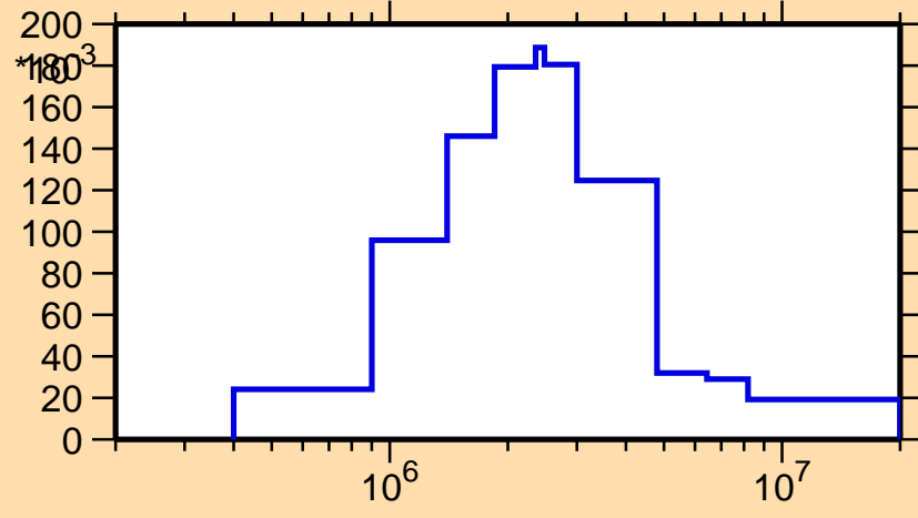
\sigma vs. E for ^{108}\text{Mo}(n,n_2)
