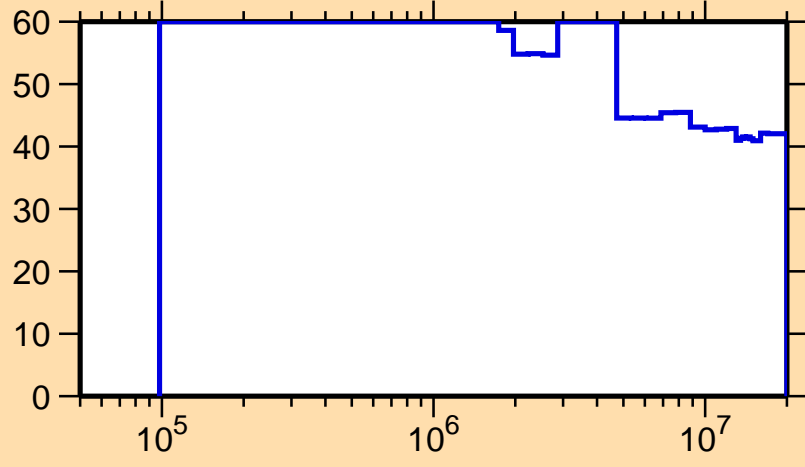
\Delta\sigma/\sigma vs. E for ^{277}_1
