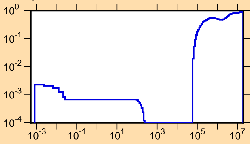
\mu vs. E for ^{278}
