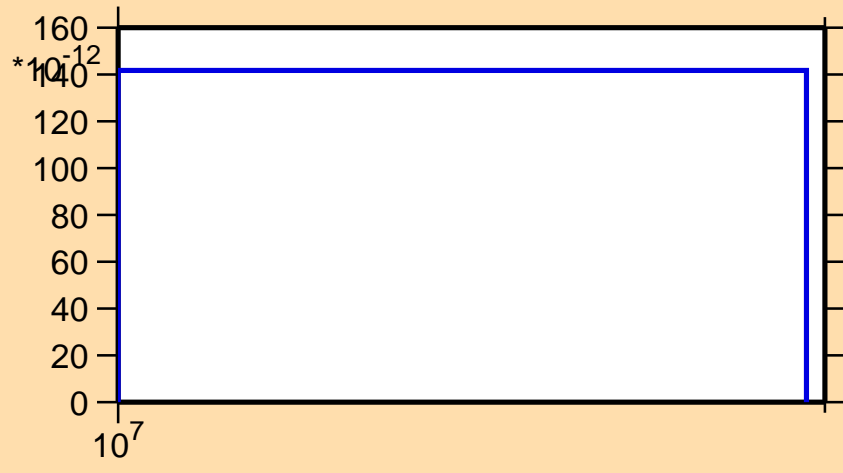
\sigma vs. E for ^{278}\alpha )
