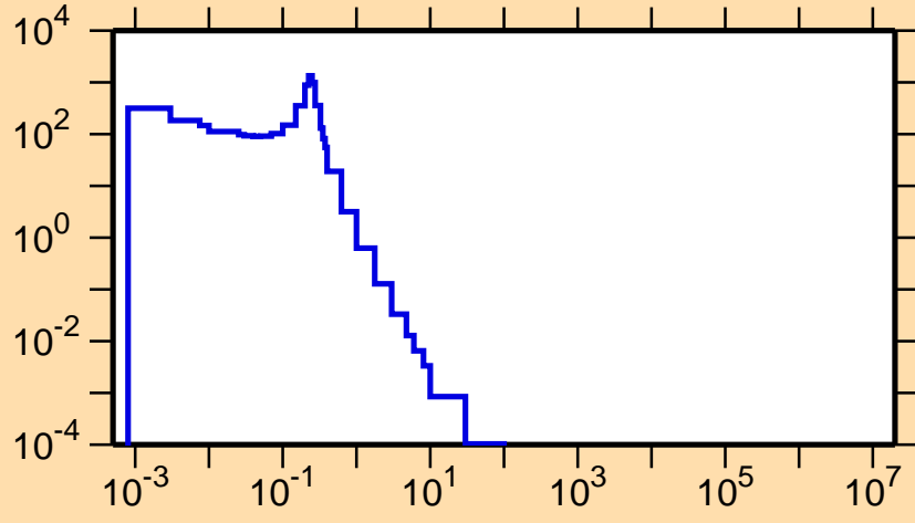
\sigma vs. E for ^{278}\gamma
