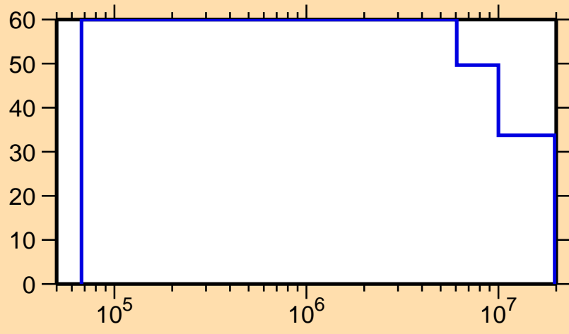
\Delta\sigma/\sigma vs. E for ^{279}_1
