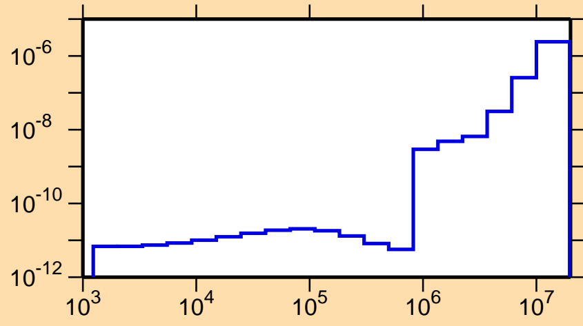
\sigma vs. E for ^{279}\alpha
