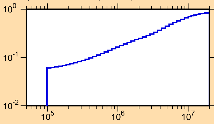
\mu vs. E for ^{13}\text{N}(\text{mt251})
