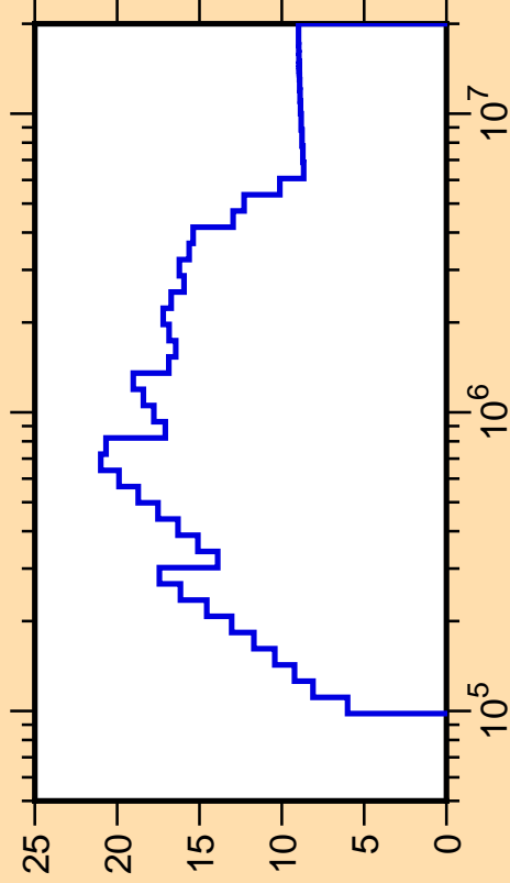
\Delta\mu/\mu vs. E for ^{13}\text{N}(\text{mt251})
