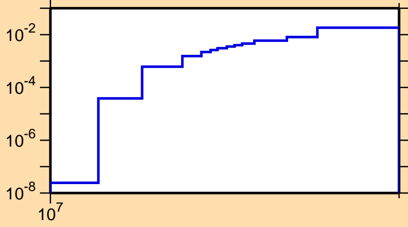
\sigma vs. E for ^{13}\text{N}(n,\alpha)
