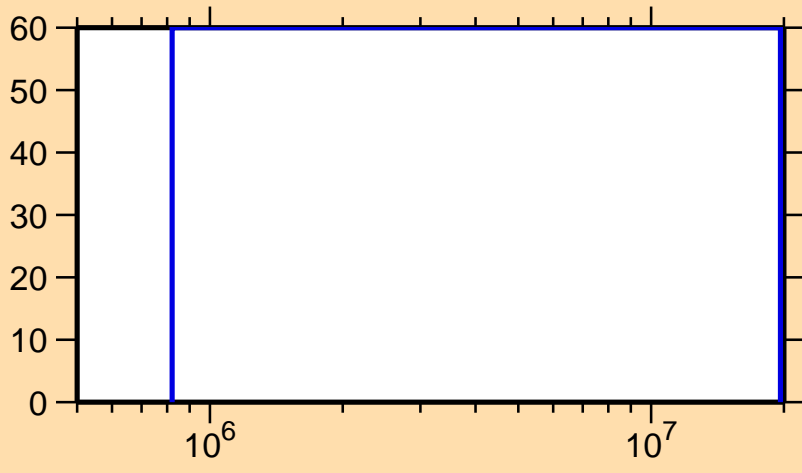
\Delta\sigma/\sigma vs. E for ^{13}\text{N}(n,\gamma)
