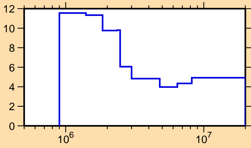
\Delta\sigma/\sigma vs. E for ^{13}\text{N}(n,\text{tot.})
