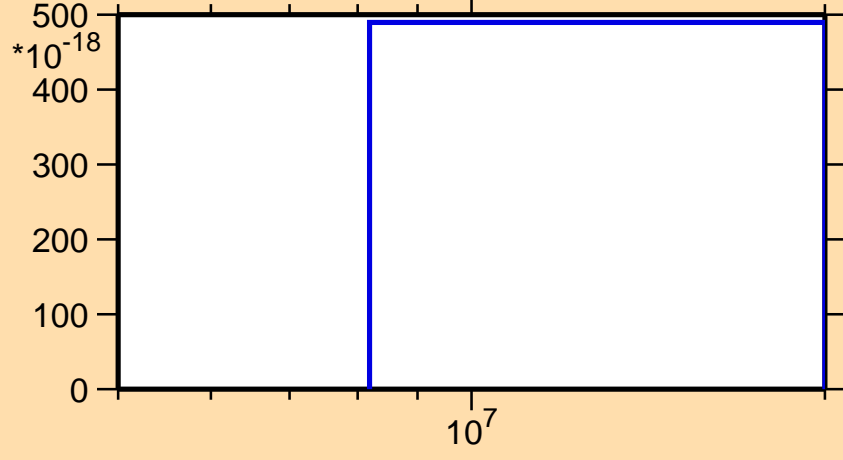
\sigma vs. E for ^{13}\text{N}(n,nd)
