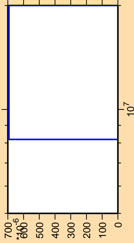
\Delta\sigma/\sigma vs. E for ^{13}\text{N}(n,nd)
