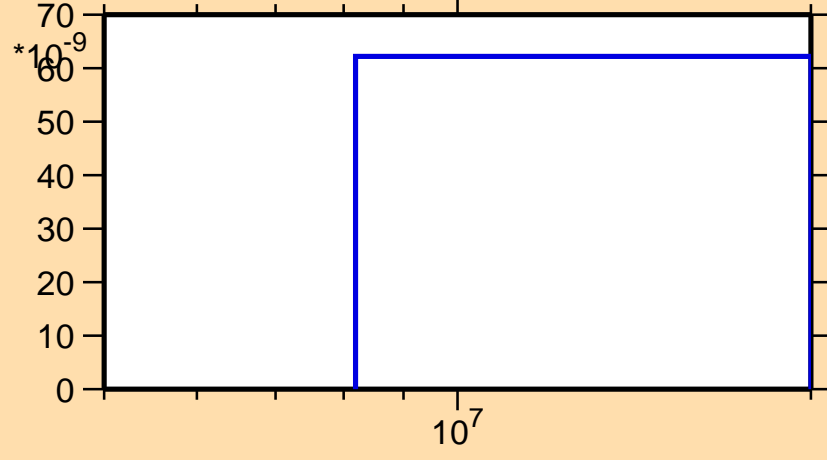
\sigma vs. E for ^{13}\text{N}(n,pd)
