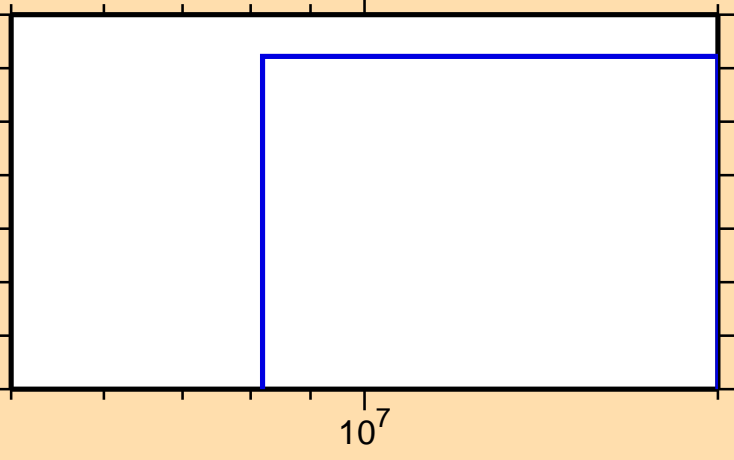
\sigma vs. E for ^{13}\text{N}(n,pd)
