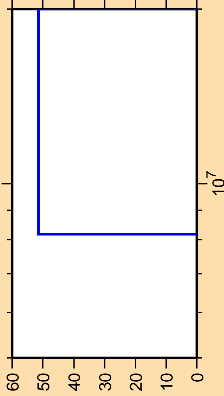
\Delta\sigma/\sigma vs. E for ^{13}\text{N}(n,t)
