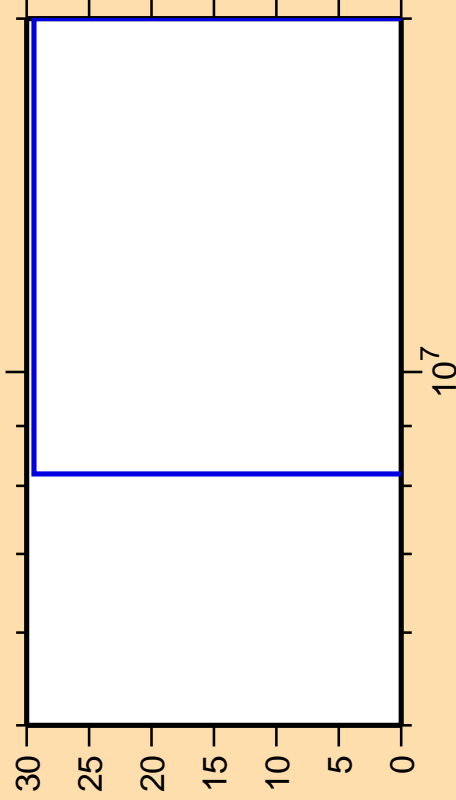
\Delta\sigma/\sigma vs. E for ^{13}\text{N}(n,pd)
