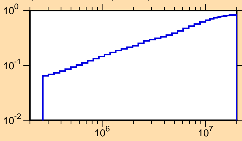
\mu vs. E for ^{16}\text{N}(\text{mt251})
