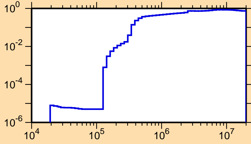
\sigma vs. E for ^{16}\text{N}(n,\text{nonel.})
