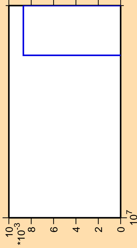
\Delta\sigma/\sigma vs. E for ^{16}\text{N}(\text{mt } 11)
