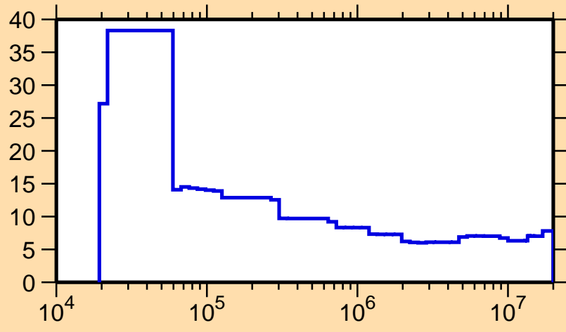
\Delta\sigma/\sigma vs. E for ^{16}\text{N}(n,\text{nonel.})
