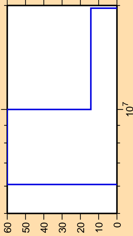
\Delta\sigma/\sigma vs. E for ^{16}\text{N}(n,2n)
