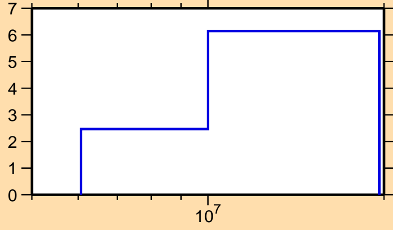
\Delta\sigma/\sigma vs. E for ^{16}\text{N}(n,el.)
