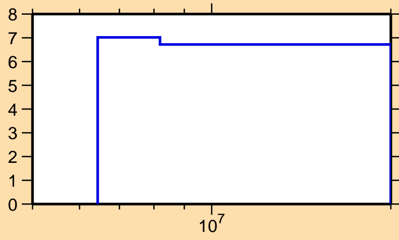
\Delta\sigma/\sigma vs. E for ^{16}\text{N}(n,nonel.)
