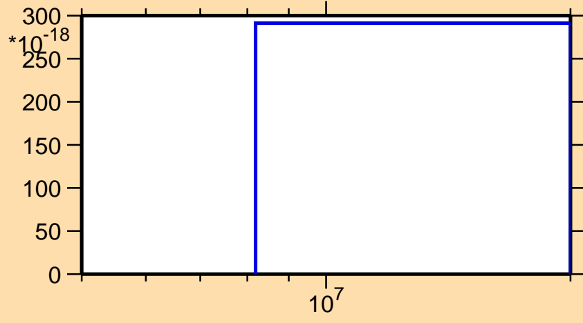
\sigma vs. E for ^{16}\text{N}(\text{mt 11})
