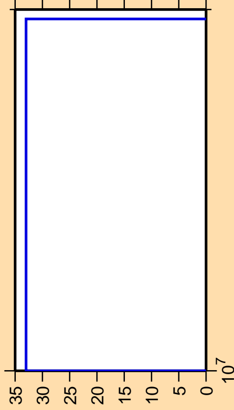
\Delta\sigma/\sigma vs. E for ^{17}\text{N}(n,nd)
