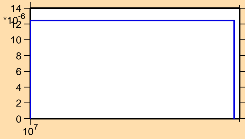
\sigma vs. E for ^{17}\text{N}(n,nd)
