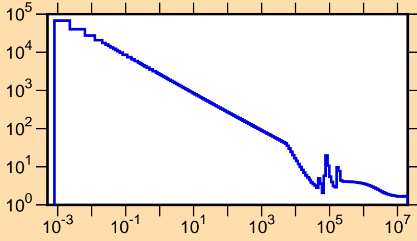
\sigma vs. E for ^{21}\text{Na}(n,\text{tot.})
