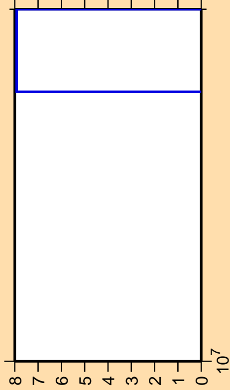
\Delta\sigma/\sigma vs. E for ^{21}\text{Na} (mt 34)
