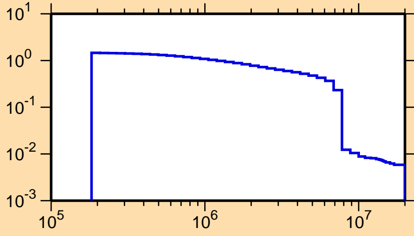
\sigma vs. E for ^{21}\text{Na}(n,p)
