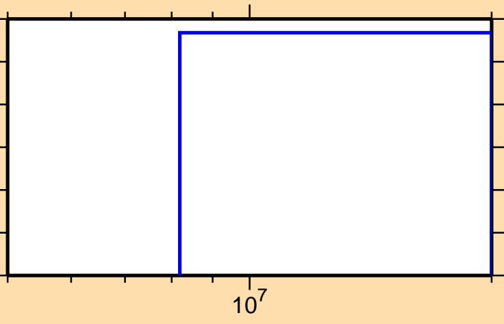
\sigma vs. E for ^{21}\text{Na}(n,\text{He}3)
