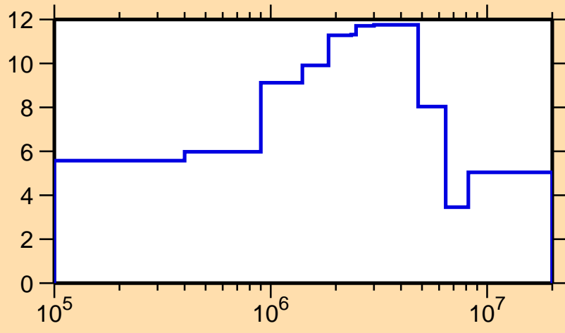
\Delta\sigma/\sigma vs. E for ^{21}\text{Na}(n,el.)
