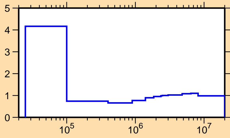
\sigma vs. E for ^{22}\text{Na}(n,\text{nonel.})
