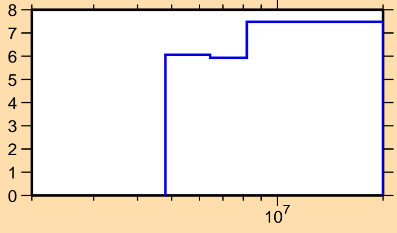
\Delta\sigma/\sigma vs. E for ^{22}\text{Na}(n,n\text{onel.})
