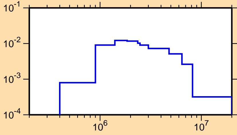
\sigma vs. E for ^{22}\text{Na}(n,n_2)
