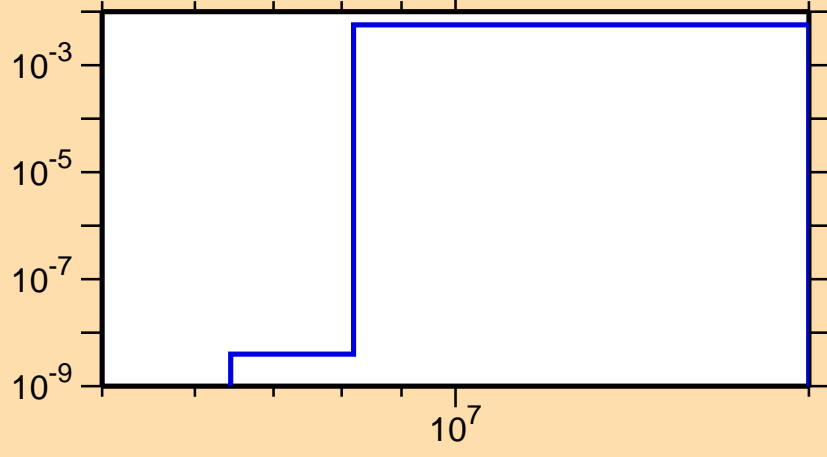
\sigma vs. E for ^{22}\text{Na}(n,p\alpha)
