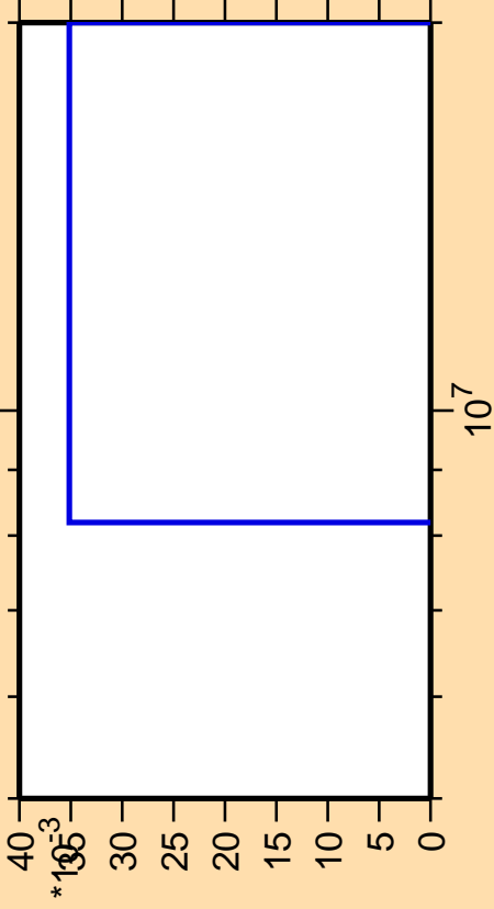
\Delta\sigma/\sigma vs. E for ^{22}\text{Na}(n,2n\alpha)
