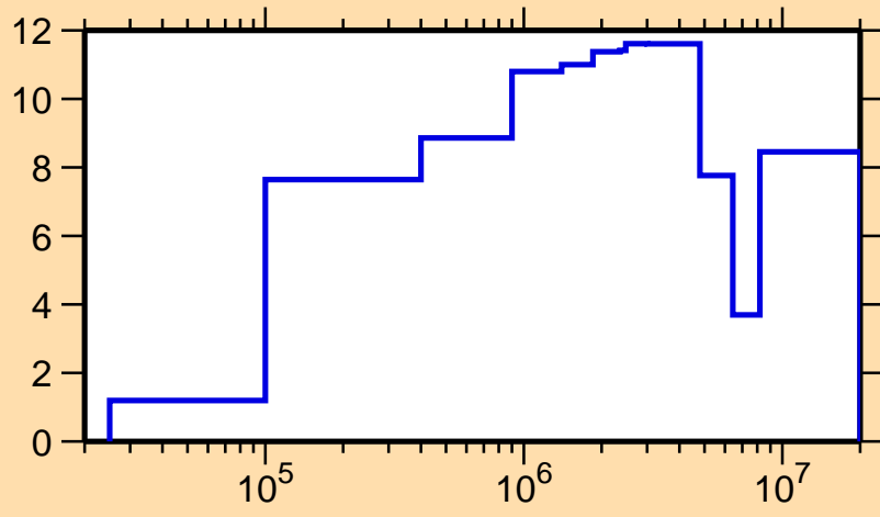
\Delta\sigma/\sigma vs. E for ^{22}\text{Na}(n,el.)
