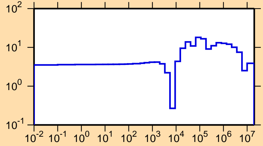
\Delta\sigma/\sigma vs. E for ^{24}\text{Na}(n,\text{tot.})
