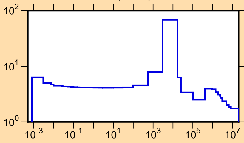
\sigma vs. E for ^{24}\text{Na}(n,\text{tot.})
