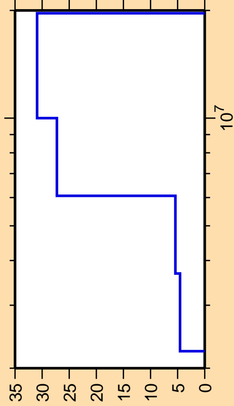
\Delta\sigma/\sigma vs. E for ^{25}\text{Na}(n,n_3)
