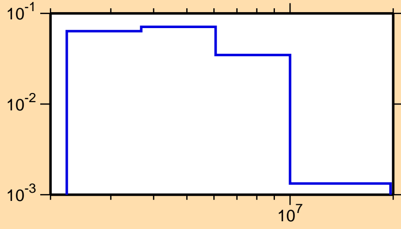
\sigma vs. E for ^{25}\text{Na}(n,n_3)
