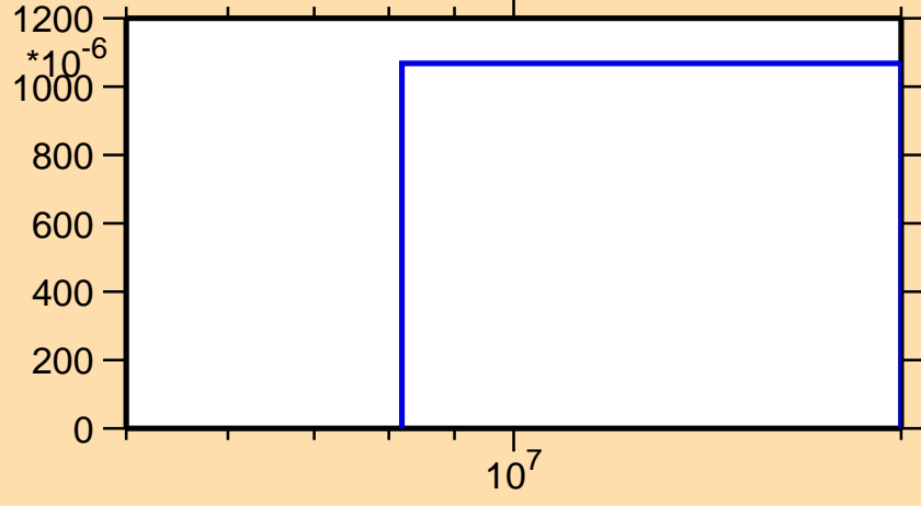
\sigma vs. E for ^{25}\text{Na}(n,np)
