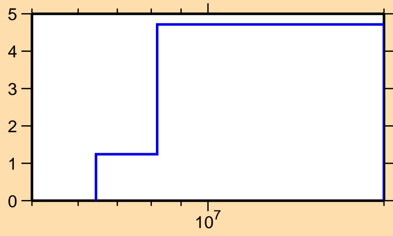
\Delta\sigma/\sigma vs. E for ^{25}\text{Na}(n,el.)
