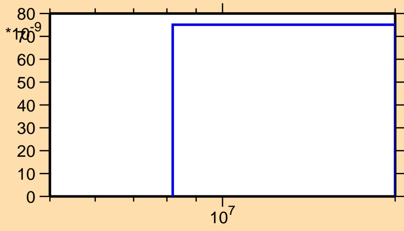
\sigma vs. E for ^{25}\text{Na}(n,nt)
