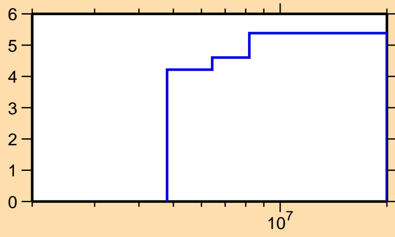
\Delta\sigma/\sigma vs. E for ^{25}\text{Na}(n,n\text{nonel.})
