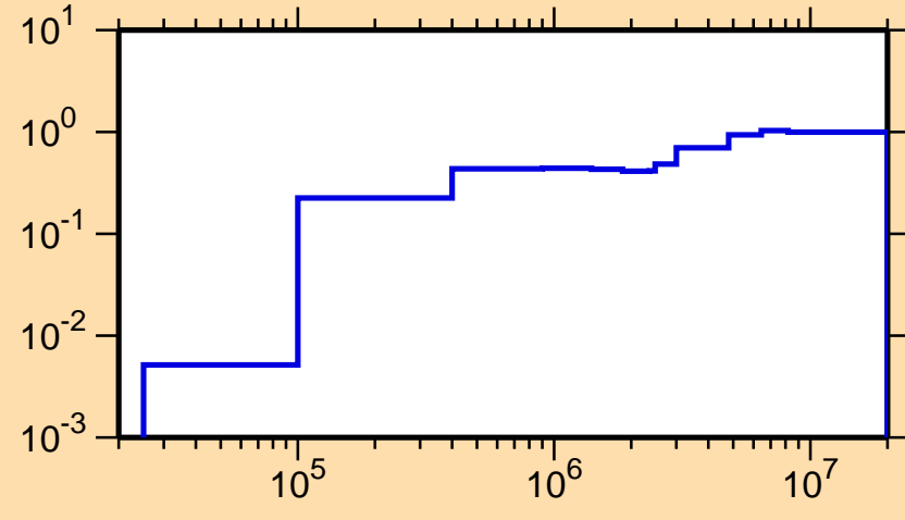
\sigma vs. E for ^{25}\text{Na}(n,\text{nonel.})
