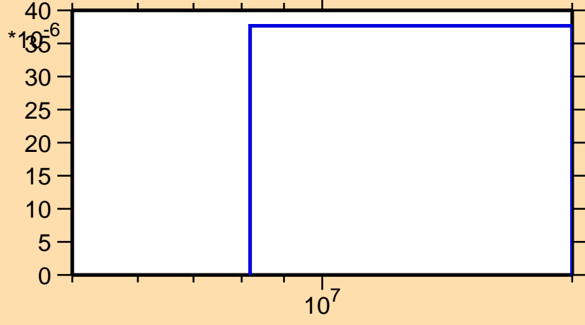
\sigma vs. E for ^{25}\text{Na}(n,3n)
