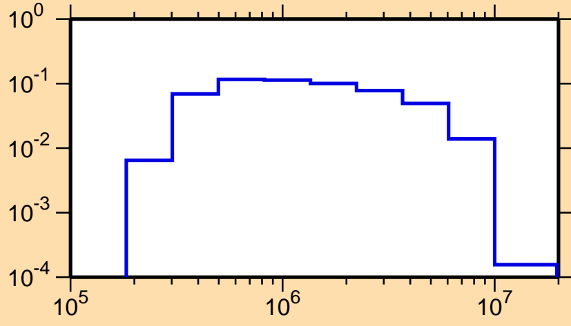
\sigma vs. E for ^{26}\text{Na}(n,n_2)
