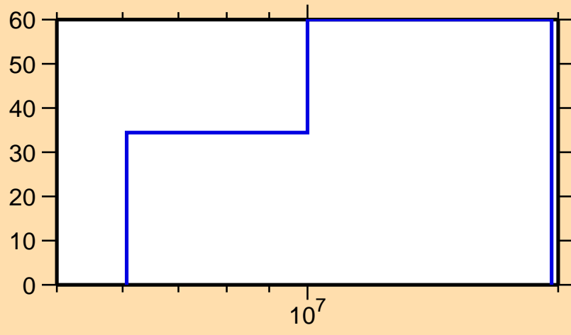
\Delta\sigma/\sigma vs. E for ^{26}\text{Na}(n,n_1)
