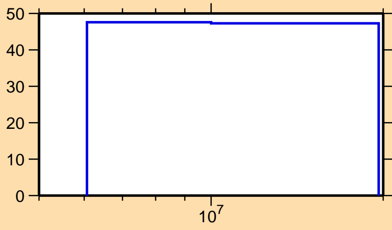
\Delta\sigma/\sigma vs. E for ^{26}\text{Na}(n,p)
