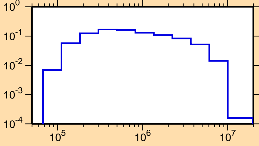
\sigma vs. E for ^{26}\text{Na}(n,n_1)
