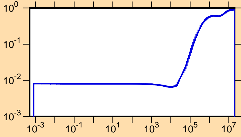
\mu vs. E for ^{83}\text{Nb}(\text{mt251})
