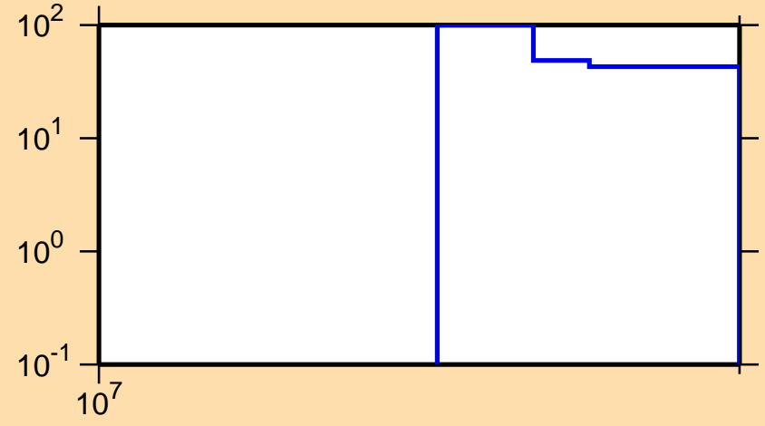
\Delta\sigma/\sigma vs. E for ^{83}\text{Nb}(n,2n)
