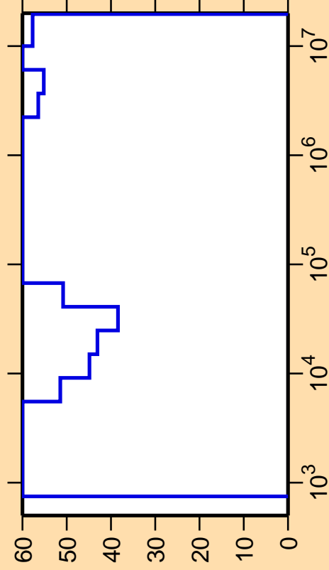
\Delta\sigma/\sigma vs. E for ^{83}\text{Nb}(n,p\alpha)
