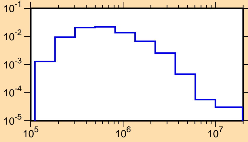
\sigma vs. E for ^{83}\text{Nb}(n,n_1)
