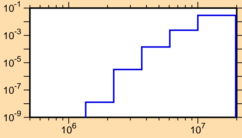
\sigma vs. E for ^{83}\text{Nb}(n,d)
