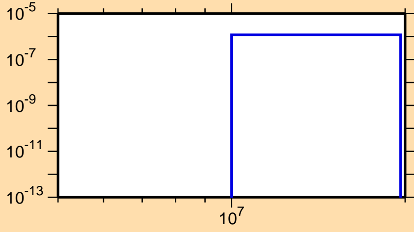
\sigma vs. E for ^{83}\text{Nb} (mt 45)
