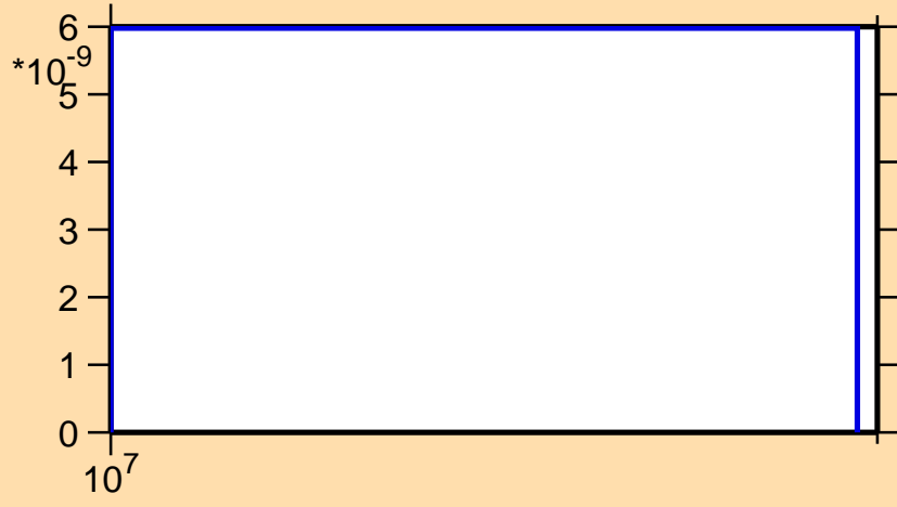
\sigma vs. E for ^{83}\text{Nb}(n,\text{nd})
