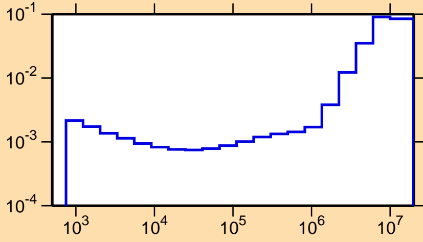
\sigma vs. E for ^{83}\text{Nb}(n,\alpha)
