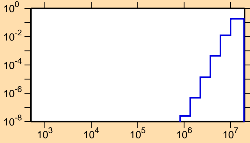
\sigma vs. E for ^{83}\text{Nb}(n,p\alpha)
