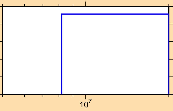
\sigma vs. E for ^{83}\text{Nb}(n,2np)
