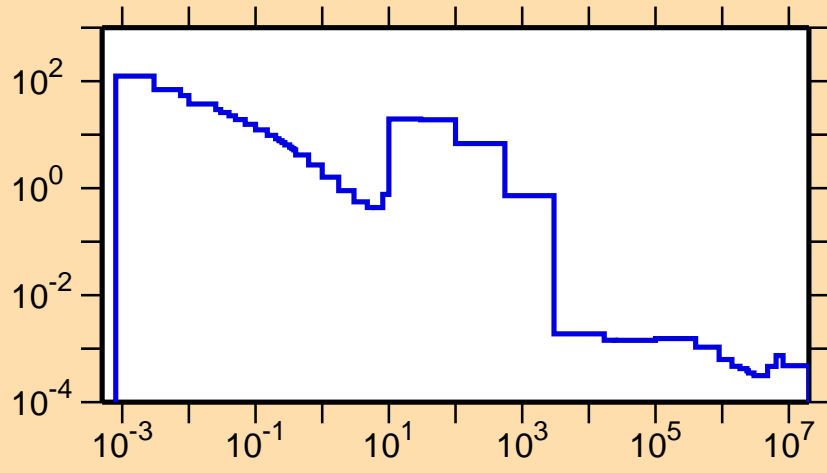
\sigma vs. E for ^{83}\text{Nb}(n,\gamma)
