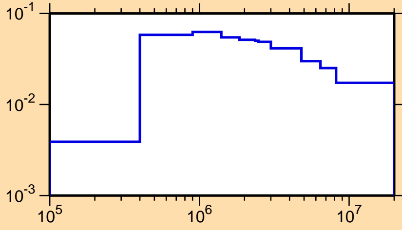
\sigma vs. E for ^{83}\text{Nb}(n,n_2)
