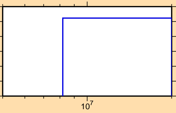
\sigma vs. E for ^{83}\text{Nb}(n,\text{nd})
