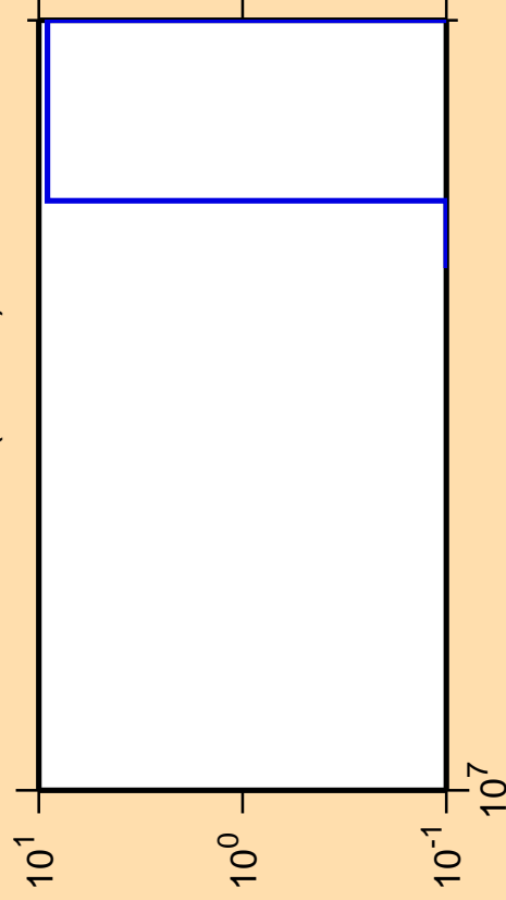
\Delta\sigma/\sigma vs. E for ^{84}\text{Nb}(n,2n\alpha)
