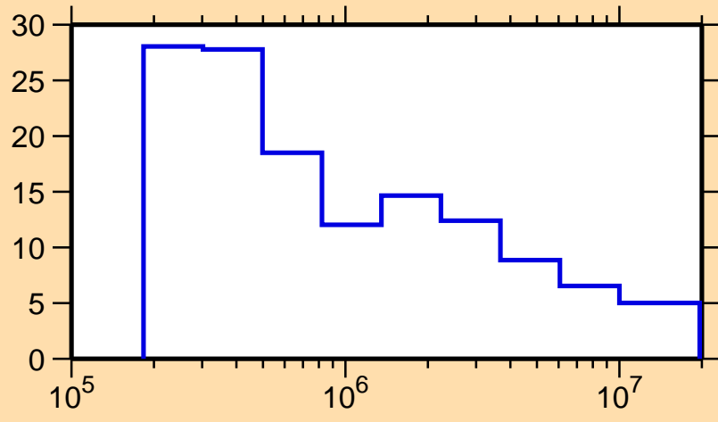
\Delta\sigma/\sigma vs. E for ^{84}\text{Nb}(n,n\text{nonel.})
