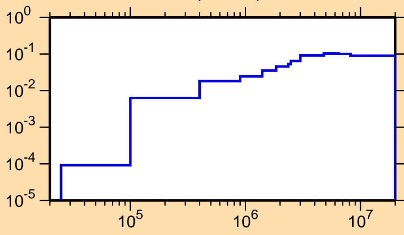
\sigma vs. E for ^{84}\text{Nb}(n,\text{inel.})
