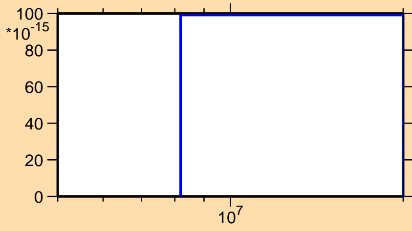
\sigma vs. E for ^{84}\text{Nb}(n,2n\alpha)
