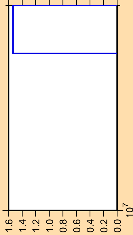
\Delta\sigma/\sigma vs. E for ^{85}\text{Nb}(n,nt)
