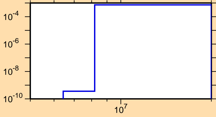
\sigma vs. E for ^{85}\text{Nb}(n,n\alpha)
