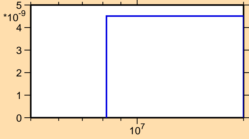
\sigma vs. E for ^{85}\text{Nb}(n,\text{nd})
