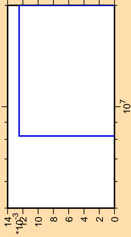
\Delta\sigma/\sigma vs. E for ^{85}\text{Nb}(n,nt)
