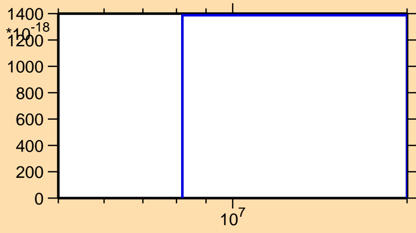
\sigma vs. E for ^{85}\text{Nb}(n,nt)
