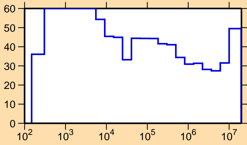
\Delta\sigma/\sigma vs. E for ^{86}\text{Nb}(n,p)
