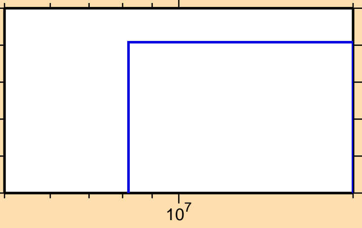
\sigma vs. E for ^{86}\text{Nb}(n,\text{pd})
