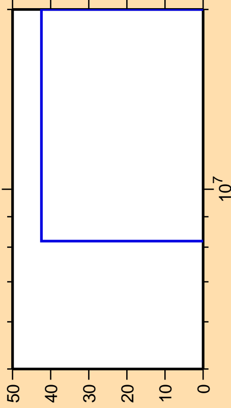
\Delta\sigma/\sigma vs. E for ^{86}\text{Nb}(n,p)
