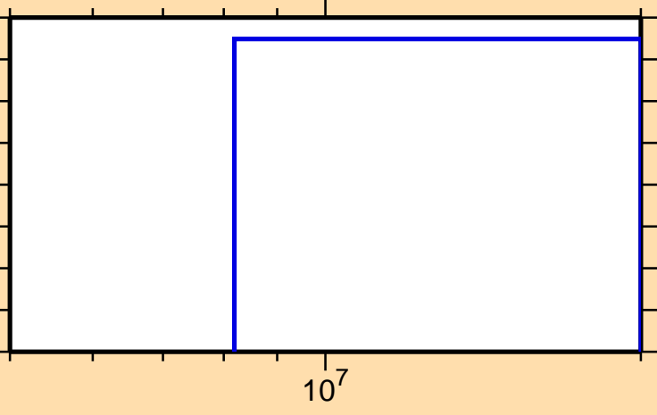
\sigma vs. E for ^{86}\text{Nb}(n,2n)
