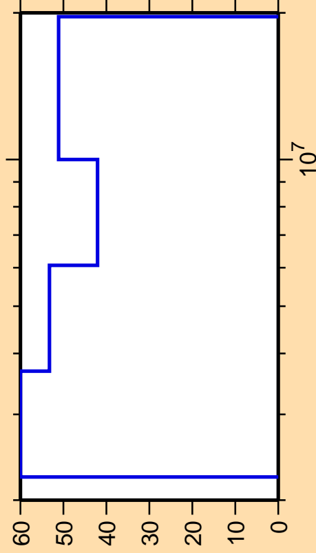
\Delta\sigma/\sigma vs. E for ^{86}\text{Nb}(n,np)
